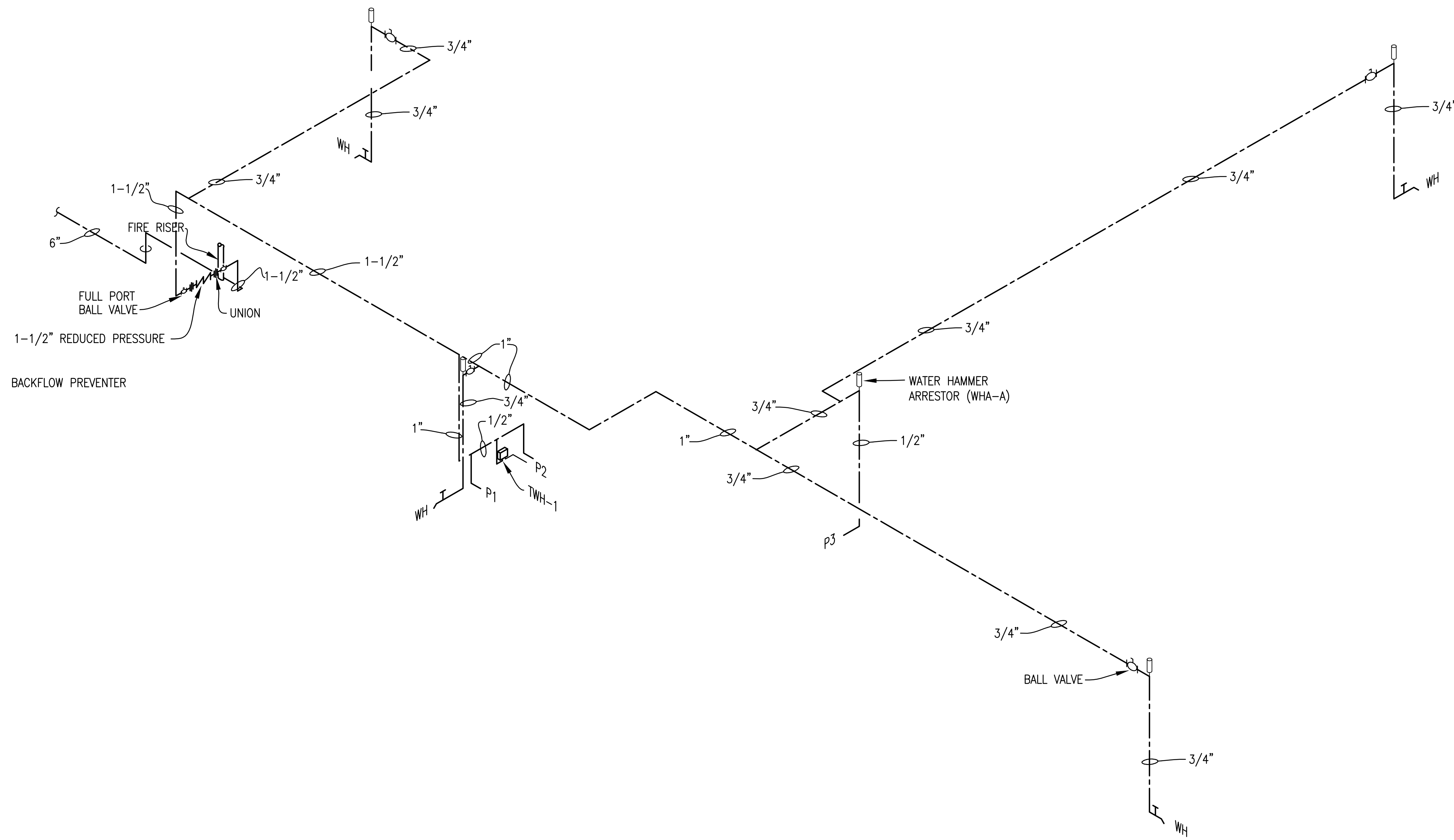
WATER RISER DIAGRAM NOT TO SCALE
