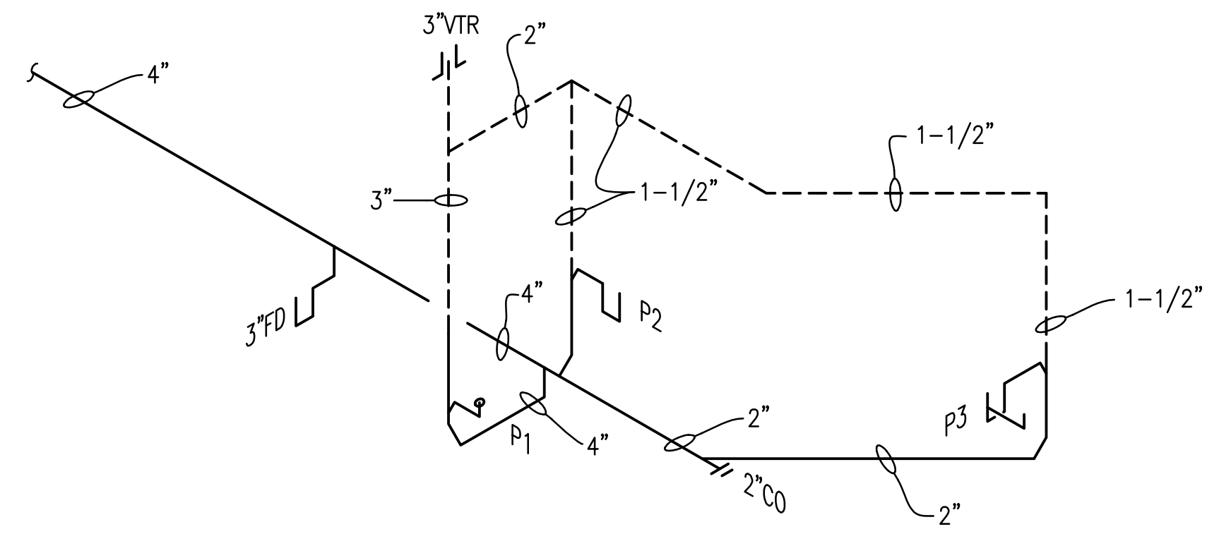
WASTE AND VENT RISER DIAGRAM NOT TO SCALE
