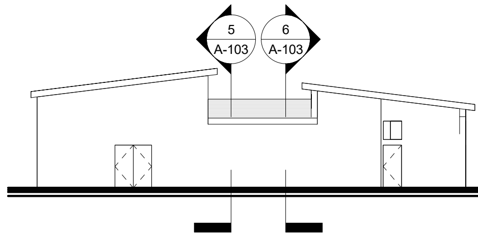
2 NORTH ELEVATION 1/16" = 1'-0"
