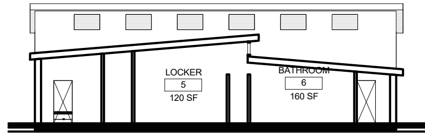
5 SECTION 01 1/16" = 1'-0"
