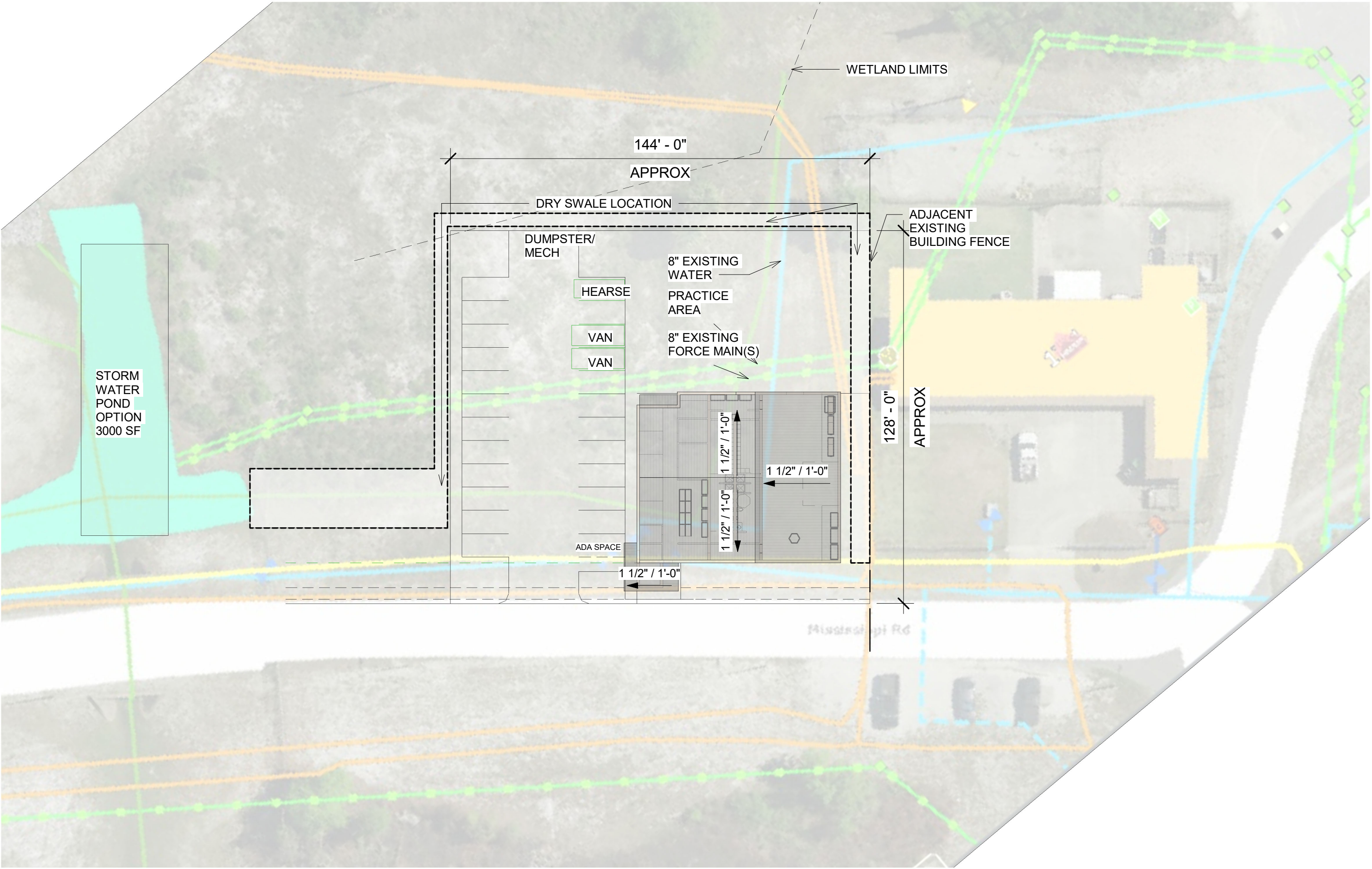
1 SITE PLAN 1" = 30'-0"
